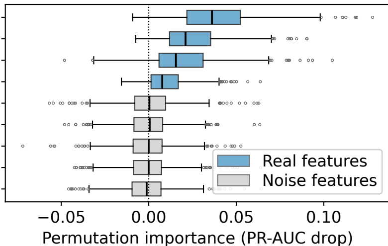
(a) Pairwise + noise
