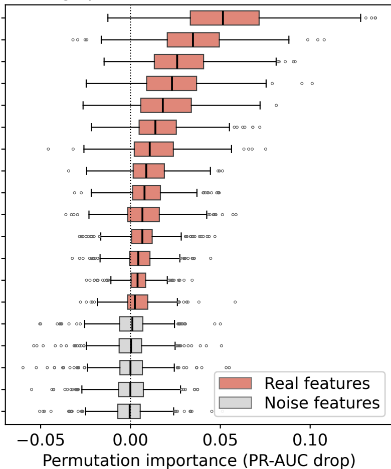
(b) Hb-graph + noise
